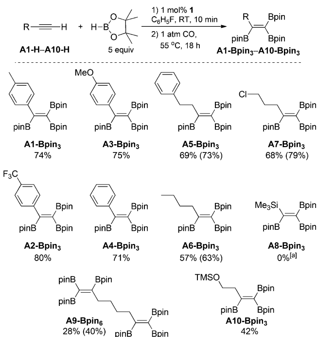
Scheme 2. Substrate scope of one-pot diboration of alkynylboronates. Reaction conditions: 1 (0.020 mmol) and HBpin (10 mmol) were dissolved in PhF in a PTFE-valved gas-tight flask. Alkyne (2.00 mmol for monoynes [1.00 mmol for 1,7-octadiyne]) was then added in 4 portions with 1 min intervals at RT. After 10 min, the mixture was degassed, refilled with 1 atm of CO, and heated at 55 °C for 18 h (see experimental for details). Yields are those of isolated products. Values within parentheses are yields determined by 1 H NMR spectroscopy. [a] 87% A8-Bpin .
